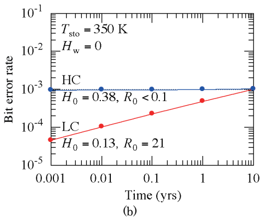
Fig. 12 (a) Bit error rate as a function of error threshold E_{th} and normalized readout field H_0 after 10 years of archiving and (b) time dependence of bit error rate during 10 years of archiving in 2 Tbps/layer 3D HAMR ( 2 \times 3 = 6 grains).
