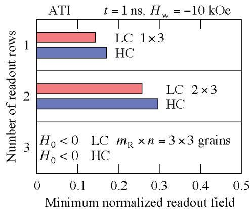
Fig. 10 Minimum normalized readout field H_0 for various numbers of readout rows m_R after AT writing in 2 Tbps/layer 3D HAMR ( 3 \times 3 = 9 grains/bit).
