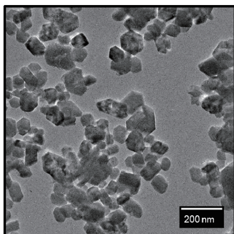
Fig. 4 TEM image of \text{MnFe}_2\text{O}_4 particles synthesized without \text{Fe}_3\text{O}_4 seed particles.
