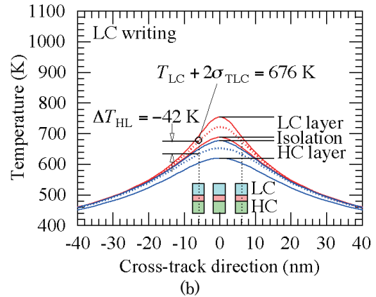
Fig. 9 Temperature profile for cross-track direction during (a) HC and (b) LC writing in 2 Tbps/layer 3D HAMR ( 3 \times 3 = 9 grains/bit).
