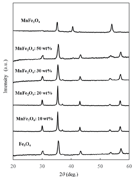
Fig. 1 XRD patterns measured in the 2\theta range of 20 to 60^\circ for \text{MnFe}_2\text{O}_4 particles, \text{Fe}_3\text{O}_4 particles, and crystallized \text{MnFe}_2\text{O}_4 (10 to 50 wt%) on the surface of \text{Fe}_3\text{O}_4 particles.
