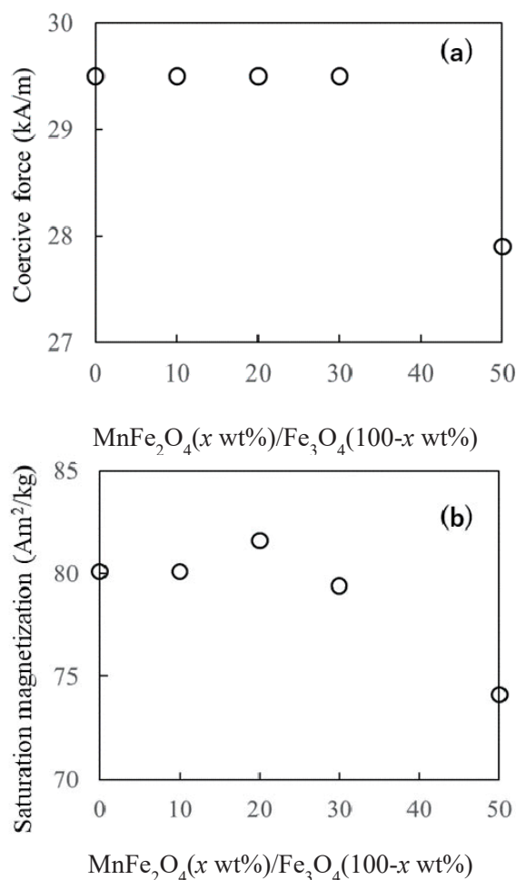
Fig. 8 Relationship between the (a) coercive force and (b) saturation magnetization, and crystallized \text{MnFe}_2\text{O}_4 content on \text{Fe}_3\text{O}_4 seed particles.
