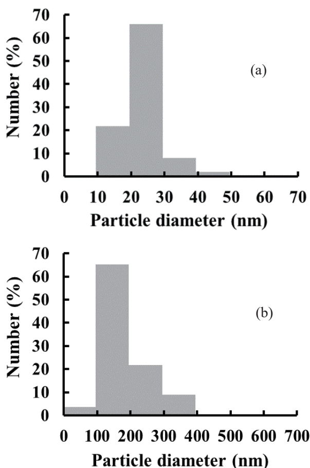
Fig. 5 Particle size distribution of \text{Fe}_3\text{O}_4 seed particles. The particle size distribution was obtained by measuring the (a) length and (b) width of approximately one hundred particles on the corresponding TEM image.
