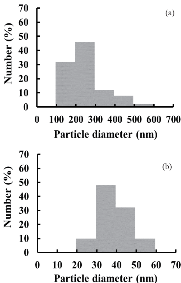
Fig. 6 Particle size distribution crystallized 30 wt% \text{MnFe}_2\text{O}_4 on \text{Fe}_3\text{O}_4 particles. The particle size distribution was obtained by measuring the (a) length and (b) width of approximately one hundred particles on the corresponding TEM image.
