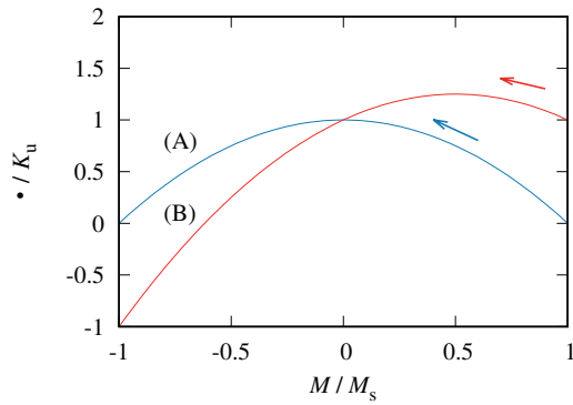
Fig. 1 Methodology for magnetization reversal on energy landscape within Ginzburg-Landau theory. (A) energy landscape of uni-axial magnetic anisotropy without an applied field, (B) under influence of an applied field.
