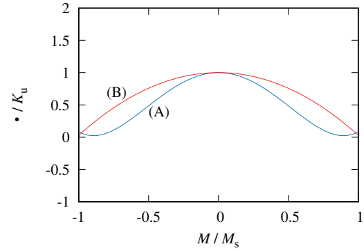
Fig. 2 Energy landscape comparison. (A) a quartic function representing the non-uniform magnetization distribution, (B) a quadratic function representing the simultaneous magnetization rotation.
