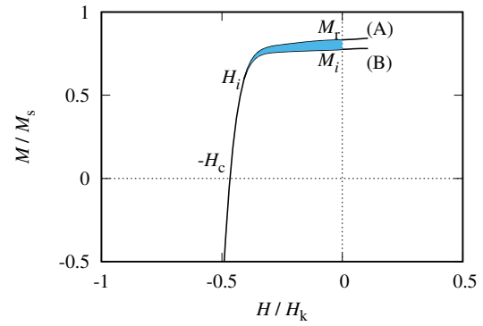
Fig. 4 Energy landscape measurement from magnetization curves. (A) a major loop forming the reference of magnetic energy, (B) a minor loop due to energy excitation. A hatched area between (A) and (B) corresponding to excitation energy by an applied field.
