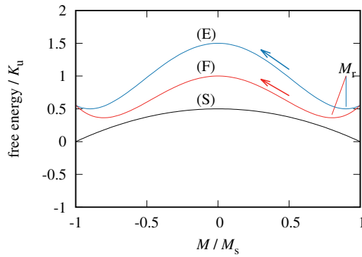
Fig. 3 Energy landscape consisting of internal energy and entropy densities. (E) shows the internal energy density given by eq.(10), (S) shows the entropy density given by eq.(18), and (F) represents the free energy density given by (F)=(E)-(S).
