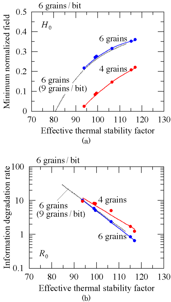
Fig. 4 (a) Minimum normalized readout field H_0 and (b) information degradation rate R_0 against effective thermal stability factor K_{\text{eff}}V/(kT) for 6 and 4 grains in 6 grains/bit.
