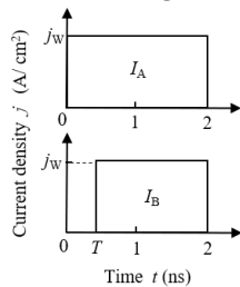
Fig. 3 Pulse diagrams of recording current applied to two metal recording wires. The current density of I_A and I_B is set so that magnetization reversal cannot occur when I_A and I_B are applied simultaneously without time difference.
