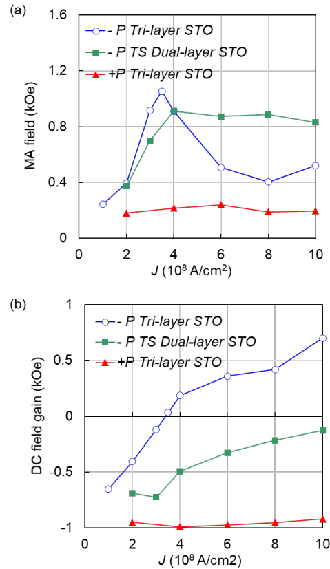
Fig. 7 Injection current dependencies of (a) MA field amplitude and (b) DC field gain, in case of negative and positive polarization tri-layer STOs and dual-layer STO with negative polarization TS.
