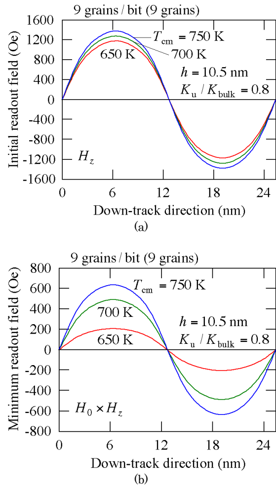
Fig. 2 (a) Initial readout field H_z and (b) minimum readout field H_0 \times H_z after 10 years of archiving for various mean Curie temperatures T_{cm} ( h = 10.5 nm and K_u/K_{bulk} = 0.8 ).
