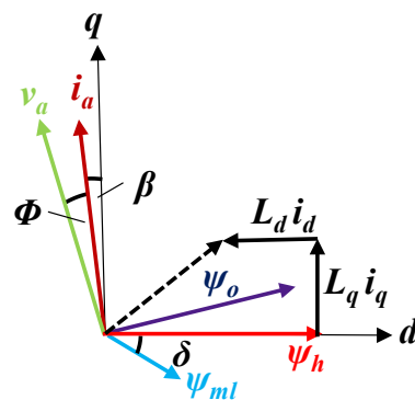
Fig. 3 Vector diagram of the IPM-type MGM.
