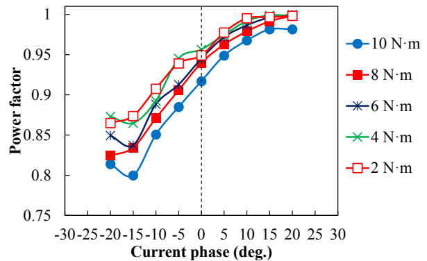
Fig. 13 Measured displacement power factor at various current phases and load torques.
