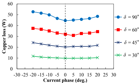
Fig. 6 Calculated copper loss at various current phases and load angles.
