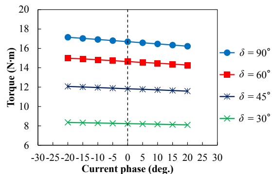
Fig. 5 Calculated torque at various current phases and load angles.
