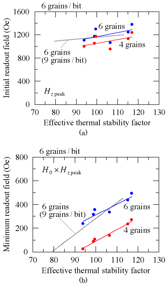
Fig. 6 (a) Initial readout field H_{z\text{peak}} and (b) minimum readout field H_0 \times H_{z\text{peak}} against effective thermal stability factor K_{\text{ueff}}V/(kT) for 6 and 4 grains in 6 grains/bit.
