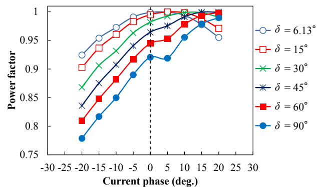
Fig. 10 Calculated displacement power factor at various current phases and load angles.
