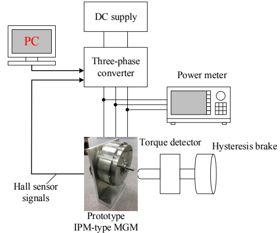
Fig. 11 Configuration of the experimental setup.
