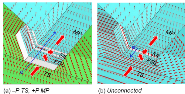
Fig. 5 Magnetization distributions near head pole tip in case of (a) negative polarization TS and positive polarization MP and (b) unconnected STO, respectively.
