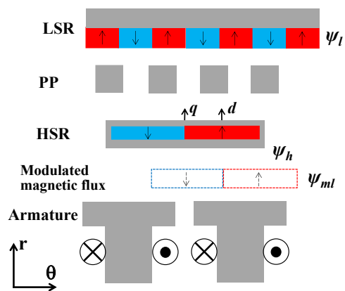
Fig. 2 Schematic diagram of the IPM-type MGM.
