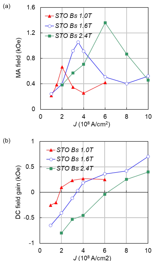
Fig. 9 Injection current dependencies of (a) MA field amplitude and (b) DC field gain, in negative polarization tri-layer STO when B_s was 1.0 T, 1.6 T, and 2.4 T.
