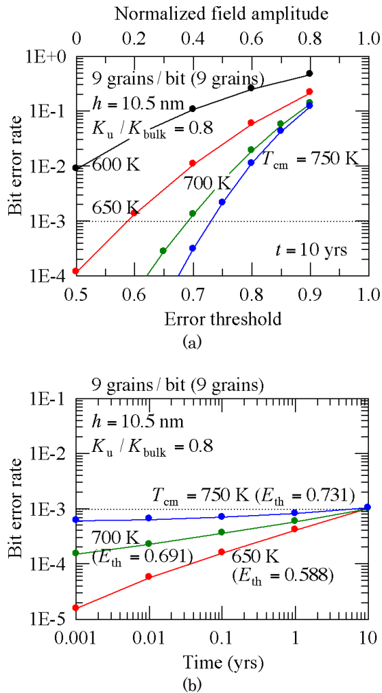
Fig. 1 (a) Bit error rate as a function of error threshold and normalized field amplitude after 10 years of archiving and (b) time dependence of bit error rate during 10 years of archiving for various mean Curie temperatures T_{cm} ( h = 10.5 nm and K_u/K_{bulk} = 0.8 ).
