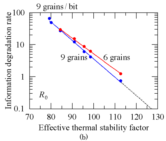
Fig. 3 (a) Minimum normalized readout field H_0 and (b) information degradation rate R_0 against effective thermal stability factor K_{ueff}V/(kT) for 9 and 6 grains in 9 grains/bit.
