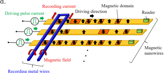
Fig. 1 Magnetic nanowire memory.
