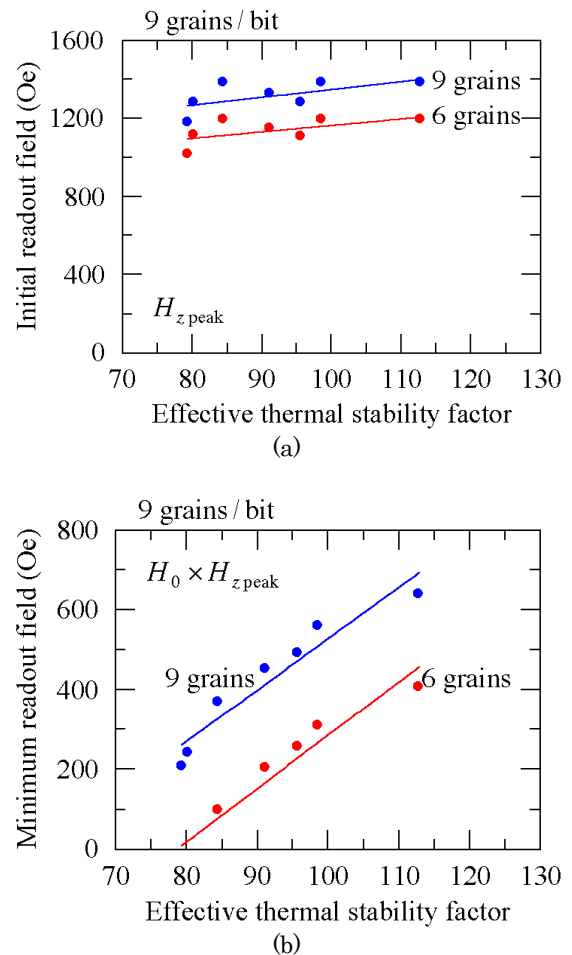
Fig. 5 (a) Initial readout field H_{z\text{peak}} and (b) minimum readout field H_0 \times H_{z\text{peak}} against effective thermal stability factor K_{\text{eff}}V/(kT) for 9 and 6 grains in 9 grains/bit.
