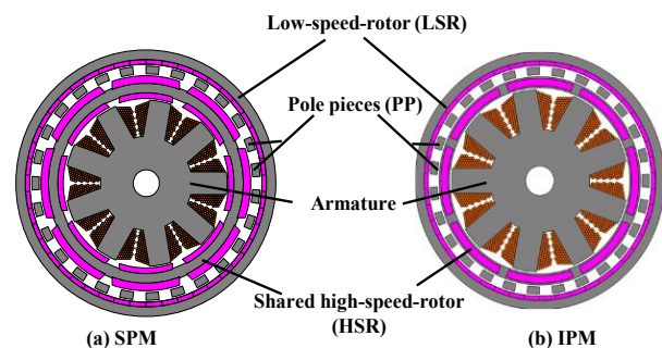
Fig. 1 Basic configuration of magnetic-geared motors (MGMs).
