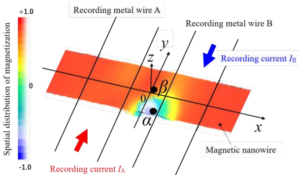
Fig. 6 Nucleation and magnetic wall propagation by recording current with the time difference T = 0.15 ns.
