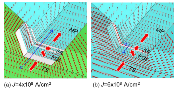
Fig. 8 Magnetization distributions near head pole tip in negative polarization tri-layer STO at injection currents of (a) J=4 \times 10^8 , and (b) J=6 \times 10^8 \text{ A/cm}^2 .
