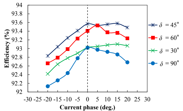
Fig. 9 Calculated efficiency at various current phases and load angles.
