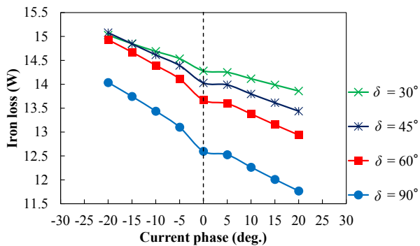
Fig. 7 Calculated iron loss at various current phases and load angles.
