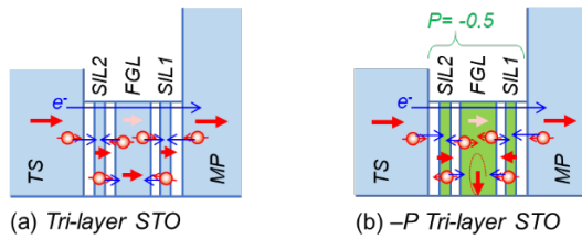
Fig. 6 Head designs of tri-layer STO made of (a) positive and (b) negative polarization materials.
