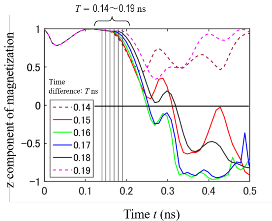
Fig. 8 Time variation of z component of magnetic moment at \alpha point.
