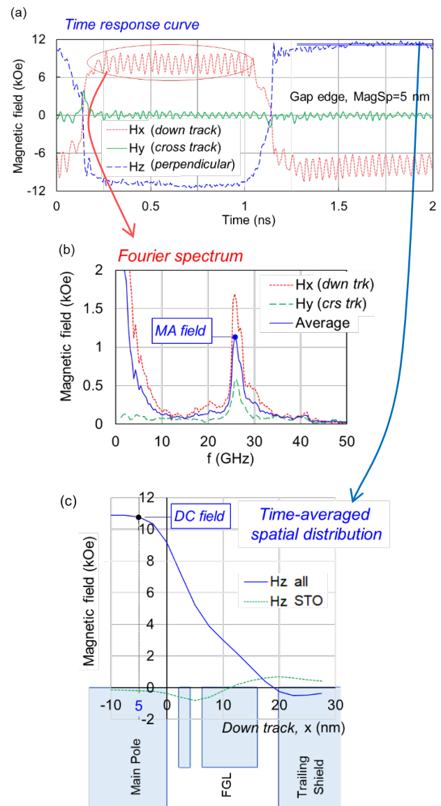
Fig. 2 (a) Time-response waveforms of writing field including STO oscillation field and (b) Fourier amplitude spectra and (c) down track profile of time-averaged perpendicular field.
