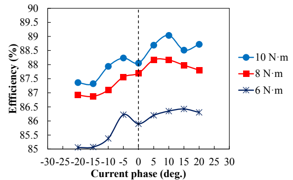
Fig. 12 Measured efficiency at various current phases and load torques.
