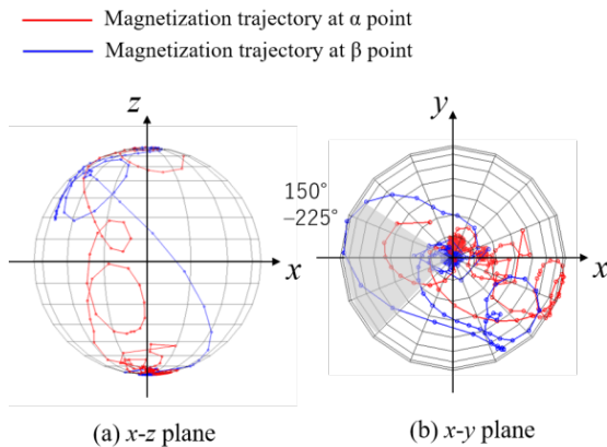
Fig. 7 Magnetization trajectory at analysis points.
