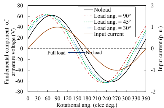
Fig. 4 Calculated waveforms of the armature voltage at various load angles.
