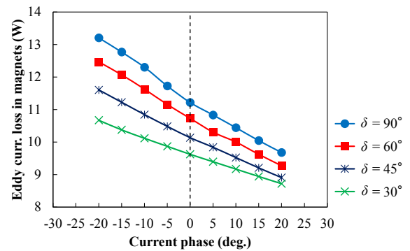
Fig. 8 Calculated eddy current loss in magnets at various current phases and load angles.
