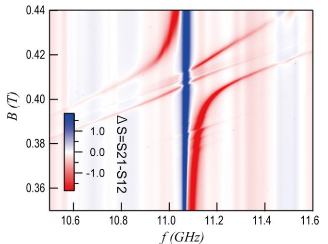
Fig. 2 Measured ferromagnetic resonance of Yttrium Iron Garnet as a function of f and B . Red(Blue) region corresponds to the right-(left-) handed circularly-polarized mode, respectively.
