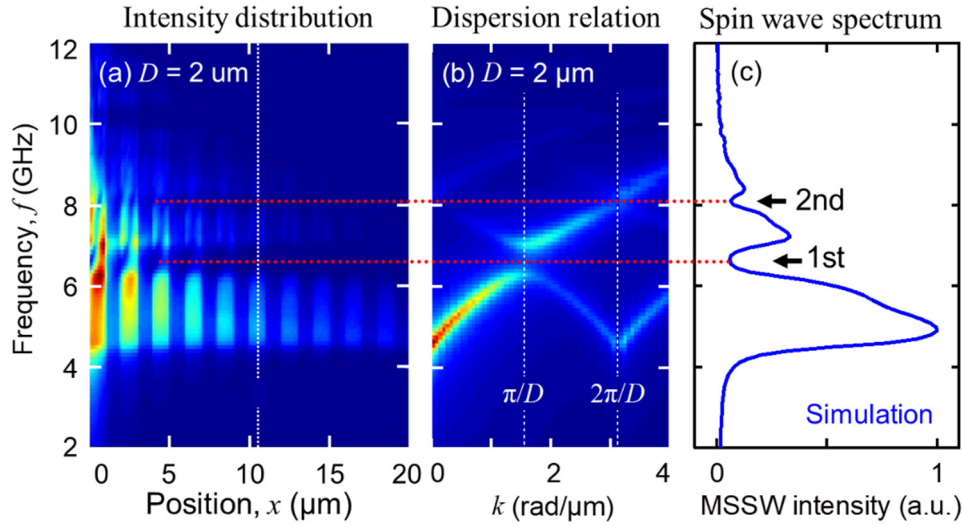
Fig. 2 Simulated intensity distribution, dispersion relation, spin wave spectrum of a Py MC with D = 2 μm.
