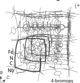
Fig. 1 Crystal structure of 1 .
