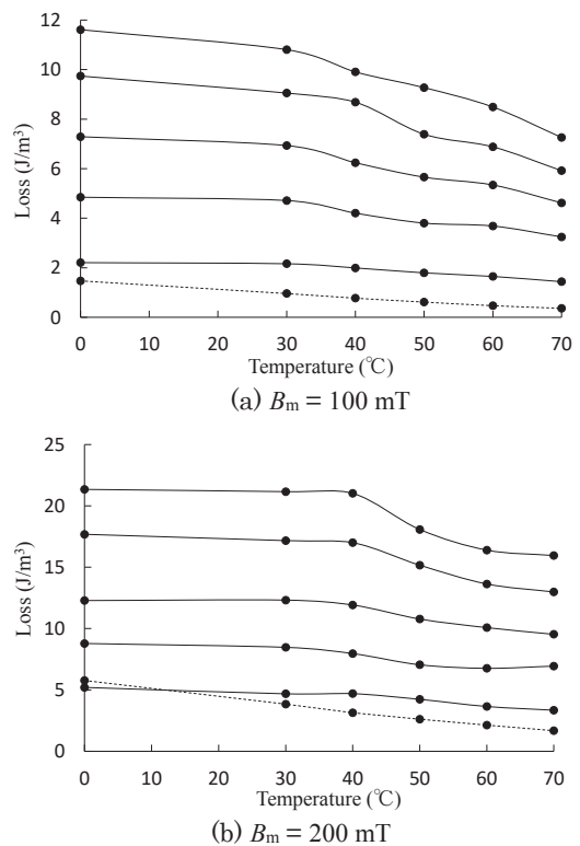
Fig. 5 Temperature characteristics of the dynamic magnetic loss with dB/dt = 1000, 800, 600, 400 and 200 \text{ mT}/\mu\text{s} from the top down, respectively. The bottom broken lines show the hysteresis losses.
