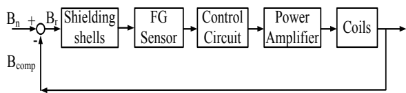
Fig. 7 A block diagram of the active shielding system
