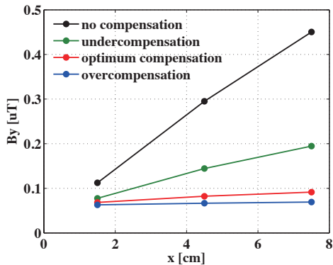
Fig. 9 Distribution of B_y component of magnetic field inside the shield for four cases: no compensation, under compensation, optimum compensation, and overcompensation
