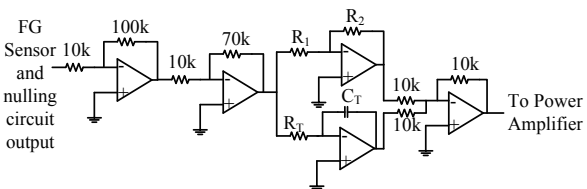
Fig. 6 Controller schematic describing the preamplifier stage and PI controller stage
